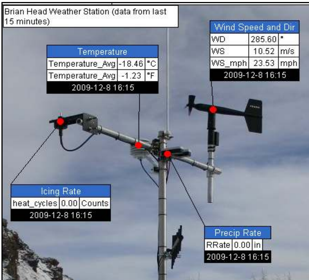
Figure 4. Sensor Suite at Brian Head
